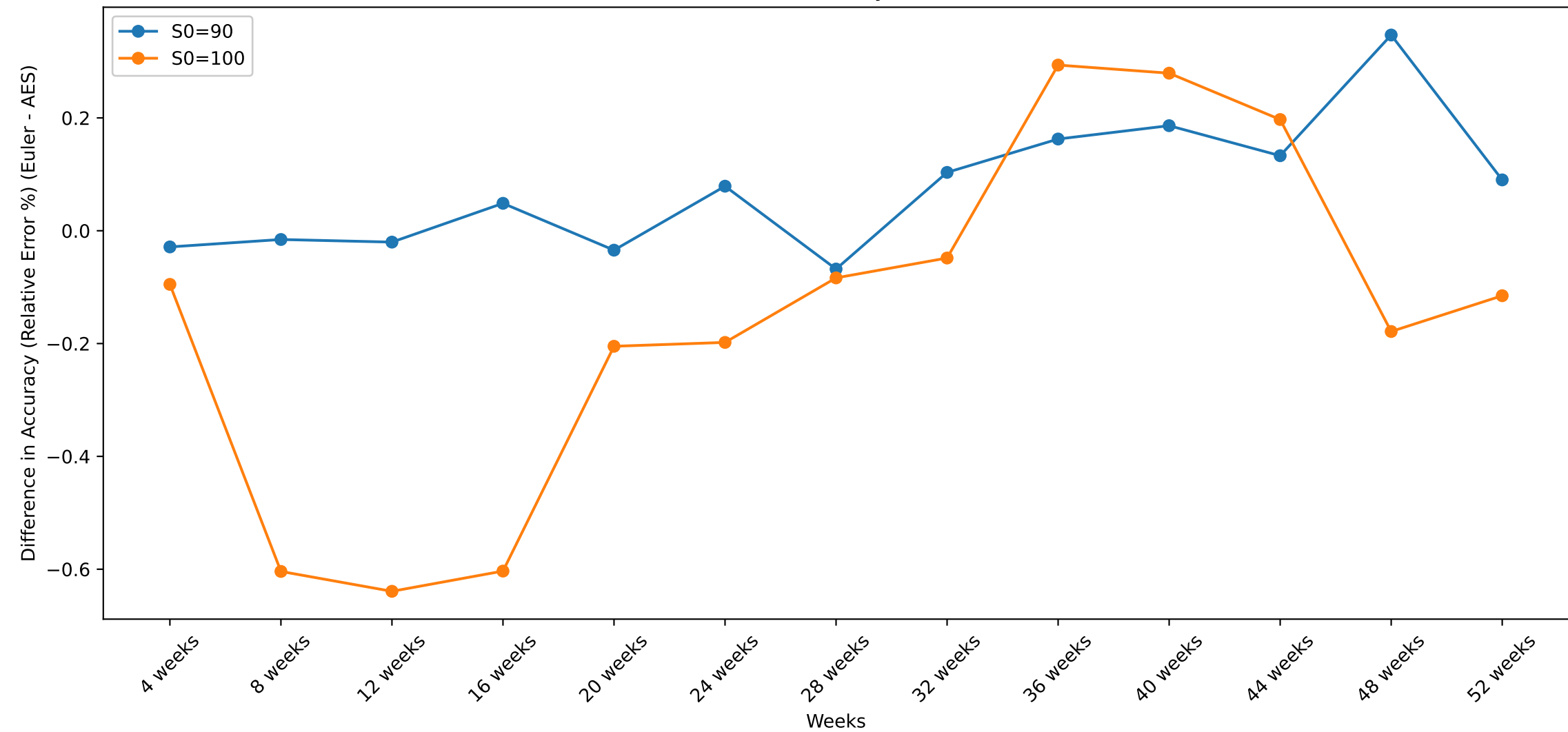
Difference in Accuracy (Euler - AES)
